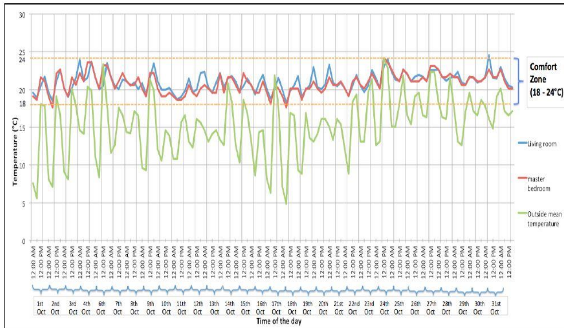
Figure 4.3: Daily temperature fluctuations comparison between living room, master bedroom and outside mean temperature at 6 hours interval for the monitoring period in the hempcrete house|
