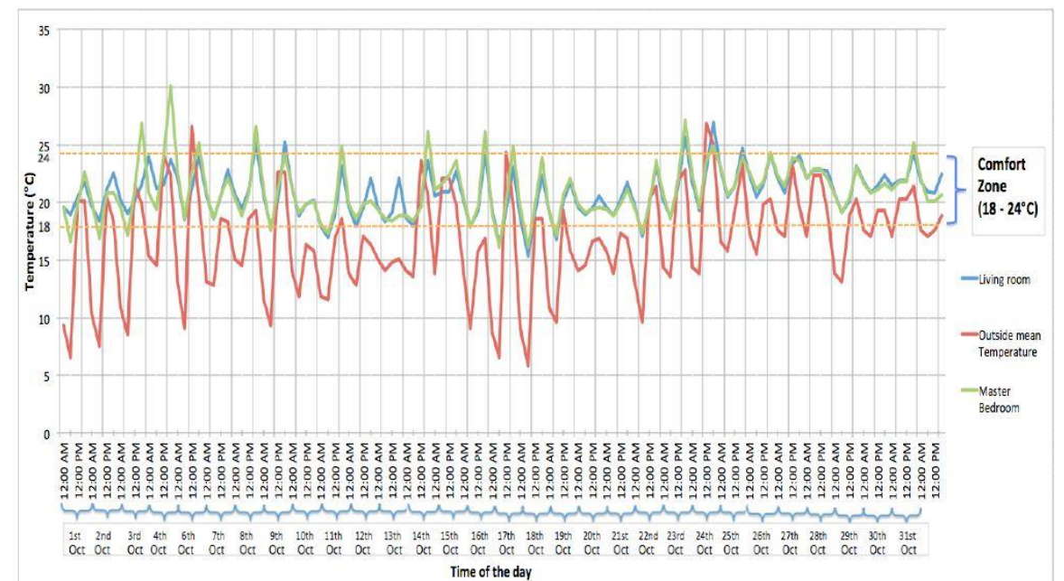
Figure 4.4: Daily temperature fluctuations comparison between living room, master bedroom and outside mean temperature at 6 hours interval for the monitoring period in the light timber frame house.
